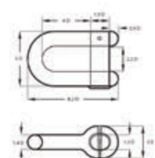
End Shackle type D
