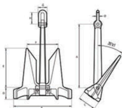
High Holding Power Anchor type "AC-14"
