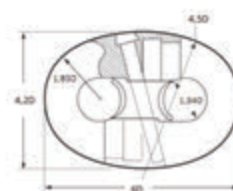
Joining Shackle Type Kenter
